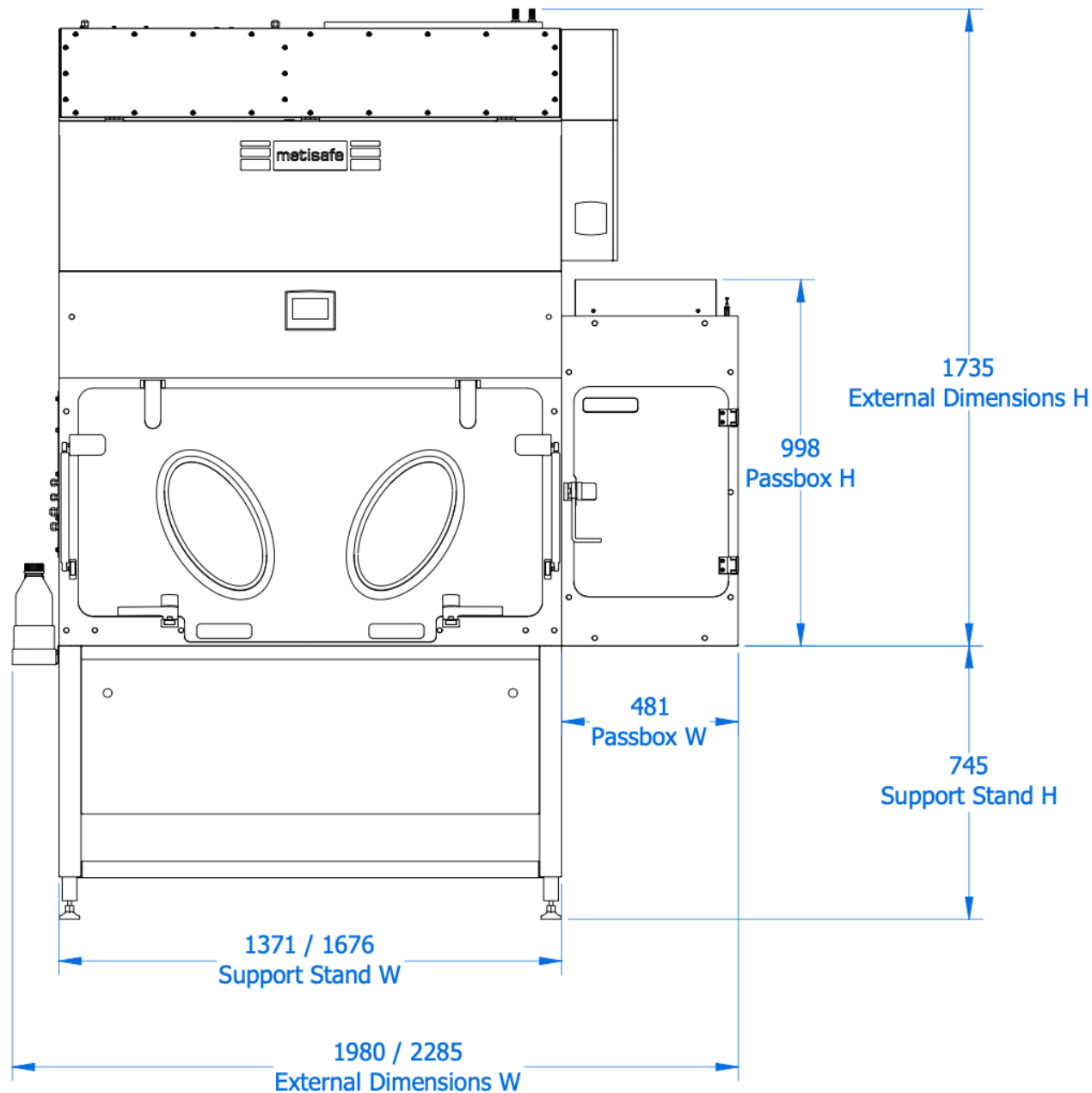
Metisafe C-Series Sterility Test Isolator
